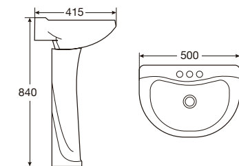
PB-326 Pedestal Basin Basin: 311011509 Pedestal: 311011517 Size: 500X415X840mm
