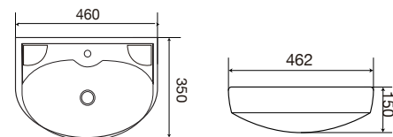
PB-018H 311011507 Wall-mounted washbasin Size: 460x350x150
