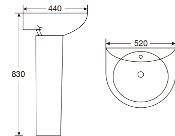
PB-828 Pedestal Basin Basin: 311011513 Pedestal: 311011517 Size: 520X440X830mm
