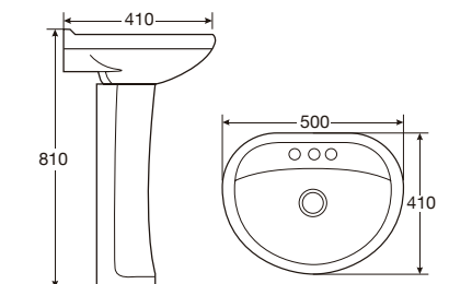
PB-207 Pedestal Basin Basin: 311011511 Pedestal: 311011519 Size: 500X410X810mm
